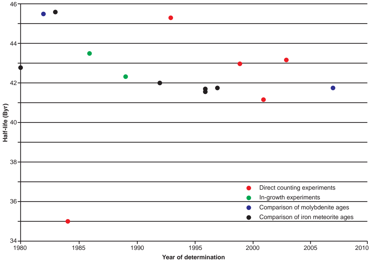
Fig. 3. Enlarged plot of the 187 Re half-life determinations since 1980 versus the year of their determination, color-coded according to the method of its determination.
