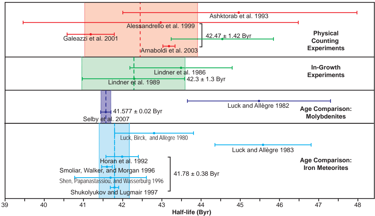
Fig. 4. Comparison of all the 187 Re half-life determinations since 1980 in the range of 41–46 Byr grouped and color-coded according to the determination method. The vertical color-shaded areas indicate the two standard deviations (2σ) from the mean values (colored vertical lines) for the groupings of determinations in each method.
