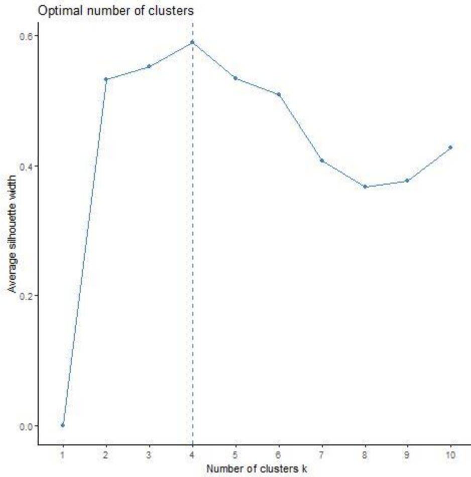
Supplementary figure 2. Silhouette plot for the Crocodylia analysis showing the average silhouette width for each cluster, calculated from the mtDNA sequence similarity matrix.
