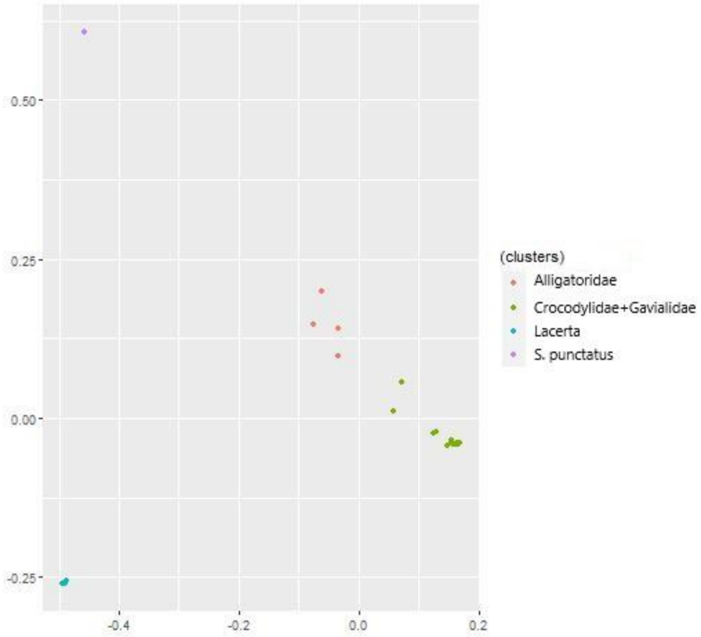
Supplementary figure 3. MDS plot for the Crocodylia analysis showing the four putative clusters in two-dimensional space.
