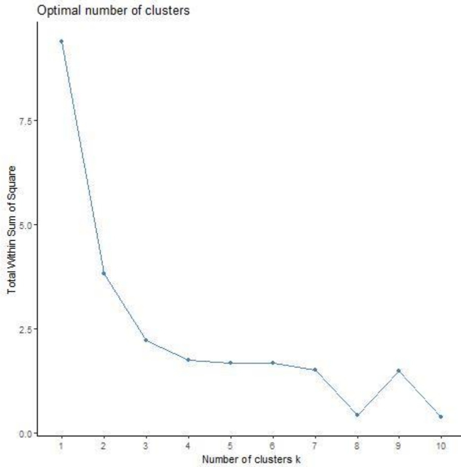
Supplementary figure 1. Elbow plot for the Crocodylia analysis showing the total within sum of squares value for each cluster, calculated from the mtDNA sequence similarity matrix.
